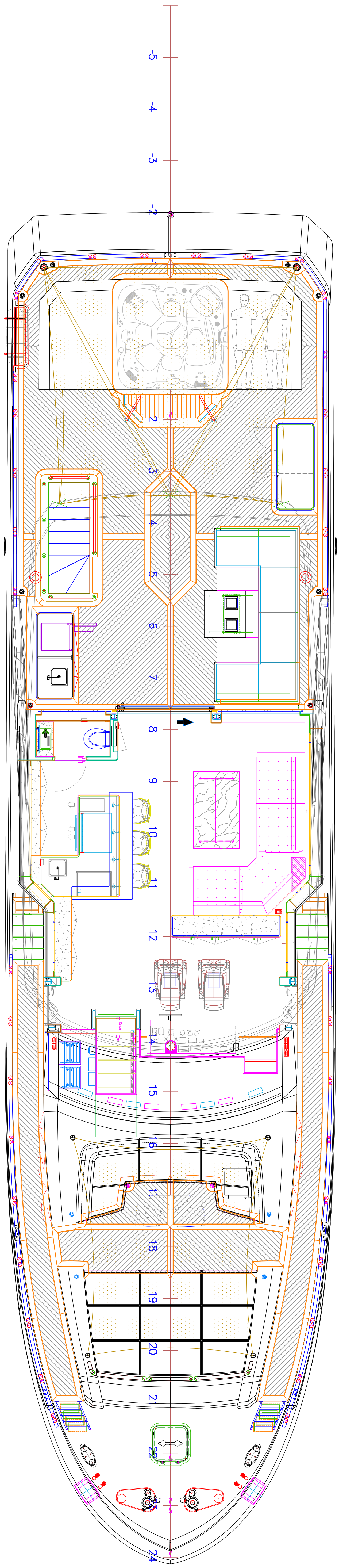
BRIDGE DECK PLAN
